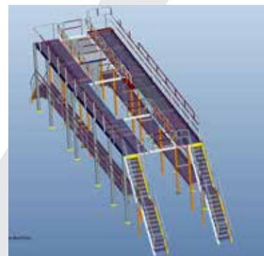
Traversing Lift Platform
